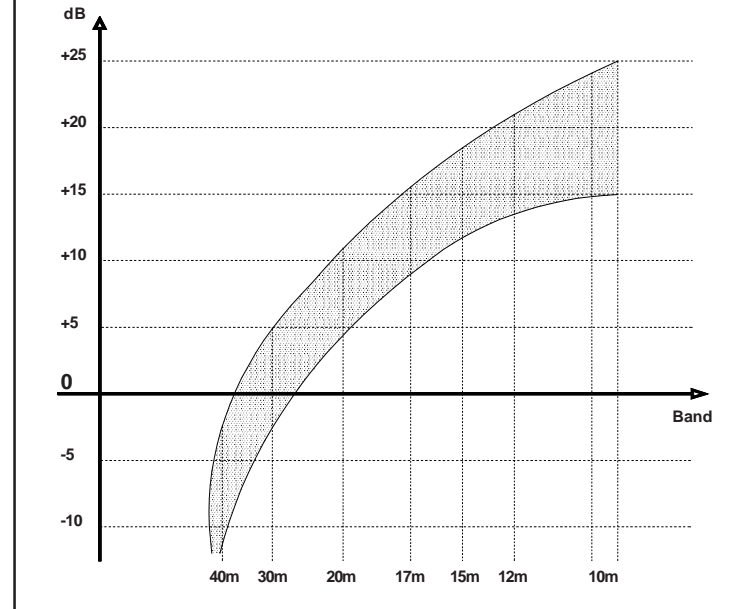
Gain versus frequency preamplifier curve chart
